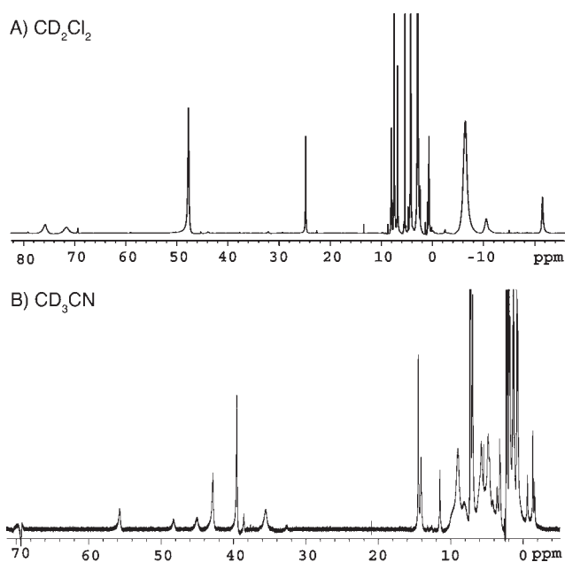
Figure 6. ^1\text{H} NMR spectra (500 MHz) of \sim 5 mM [\text{Fe}_2(\text{PIM})-(\text{Ar}^{101}\text{CO}_2)_2] ( 2 ) in solutions of (A) dichloromethane- d_2 and (B) acetonitrile- d_3 at room temperature.
