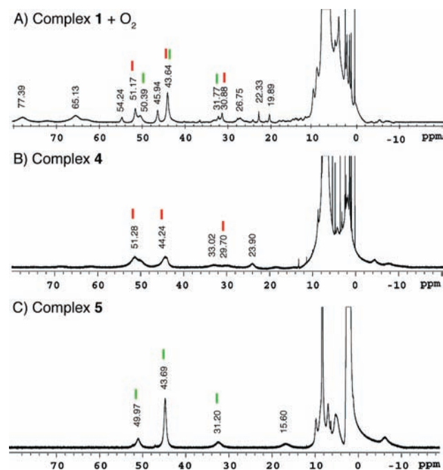
Figure 10. 1 H NMR spectra (500 MHz) of (A) [\text{Fe}_2(\text{PIM})(\text{Ph}_3\text{C}-\text{CO}_2)_2] ( 1 ) + O 2 , (B) [\text{Fe}_2(\mu\text{-OH})(\text{PIM})(\text{Ph}_3\text{CCO}_2)_3] ( 4 ), and (C) [\text{Fe}_4(\mu\text{-OH})_6(\text{PIM})_2(\text{Ph}_3\text{CCO}_2)_2] ( 5 ). Comparison of spectrum A to spectra B and C reveals that reaction of 1 with O 2 leads to formation of 4 and 5 , in addition to at least one other product. The peaks that most likely arise from 4 and 5 in spectrum A are marked with red and green lines, respectively. Not all of the peaks in A corresponding to 4 and 5 were assigned because of uncertainty due to the broadness and overlap of some resonances. All spectra were recorded at room temperature with diiron complex concentrations of ~5–10 mM in CDCl 3 . Relative peak heights are not normalized between spectra.
